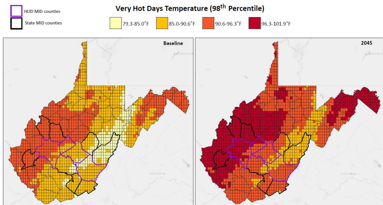
Figure 24: Temperature (°F) for a “Very Hot Day” in West Virginia.
